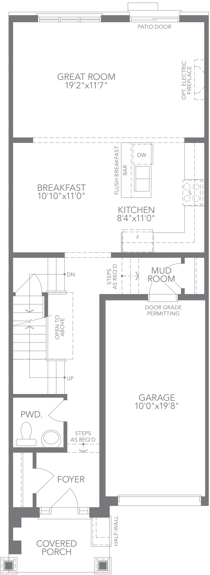
T1 - ELEV. C2 GROUND FLOOR PLAN
