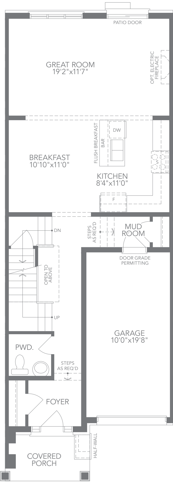
T1 - ELEV. A2 GROUND FLOOR PLAN
