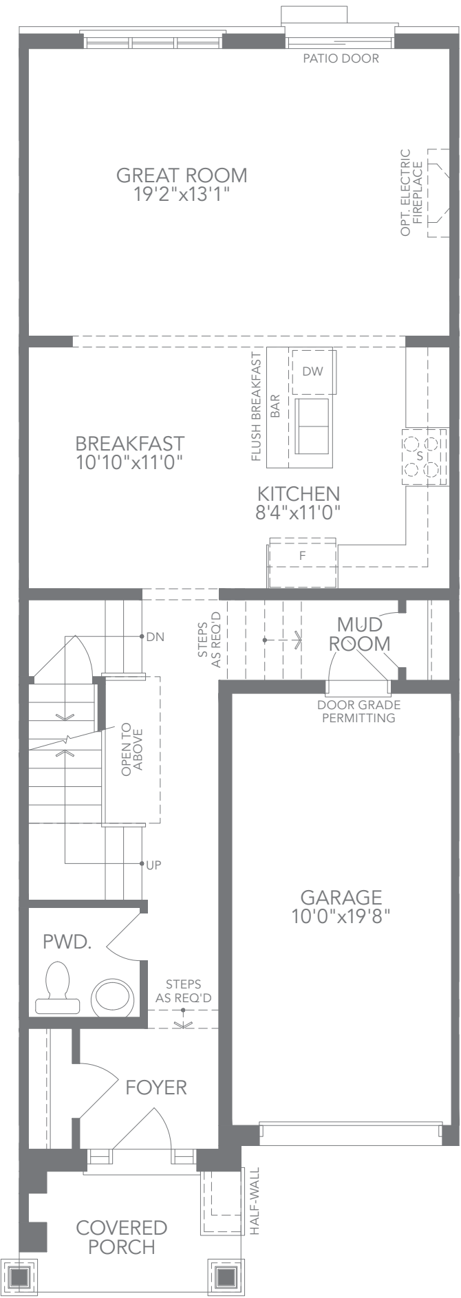
T2 - ELEV. C1 GROUND FLOOR PLAN
