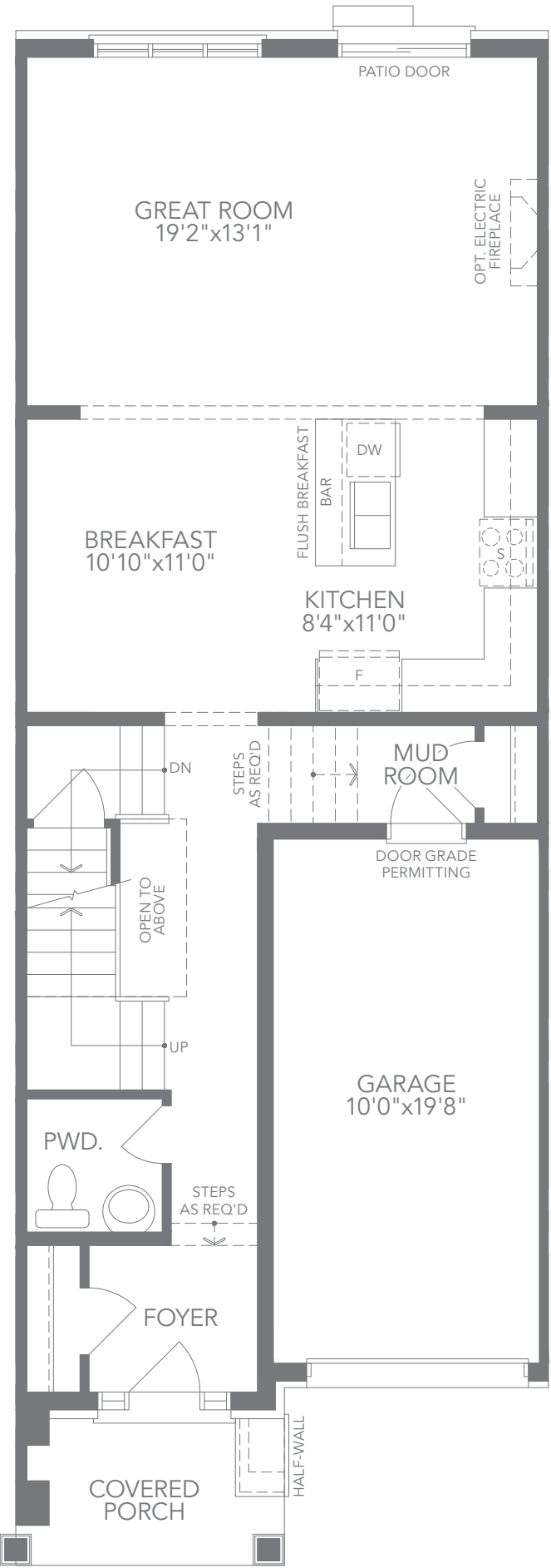
T2 - ELEV. A2 GROUND FLOOR PLAN
