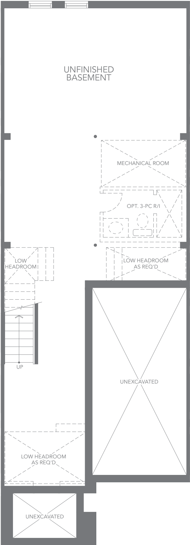
T2 - ELEV. B1 BASEMENT FLOOR PLAN
