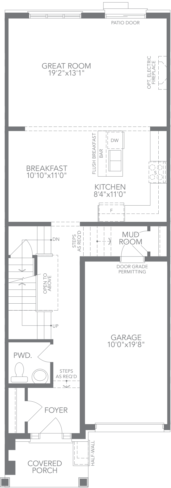
T2 - ELEV. A1 GROUND FLOOR PLAN
