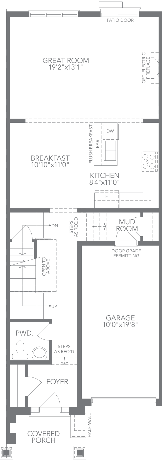
T2 - ELEV. B2 GROUND FLOOR PLAN
