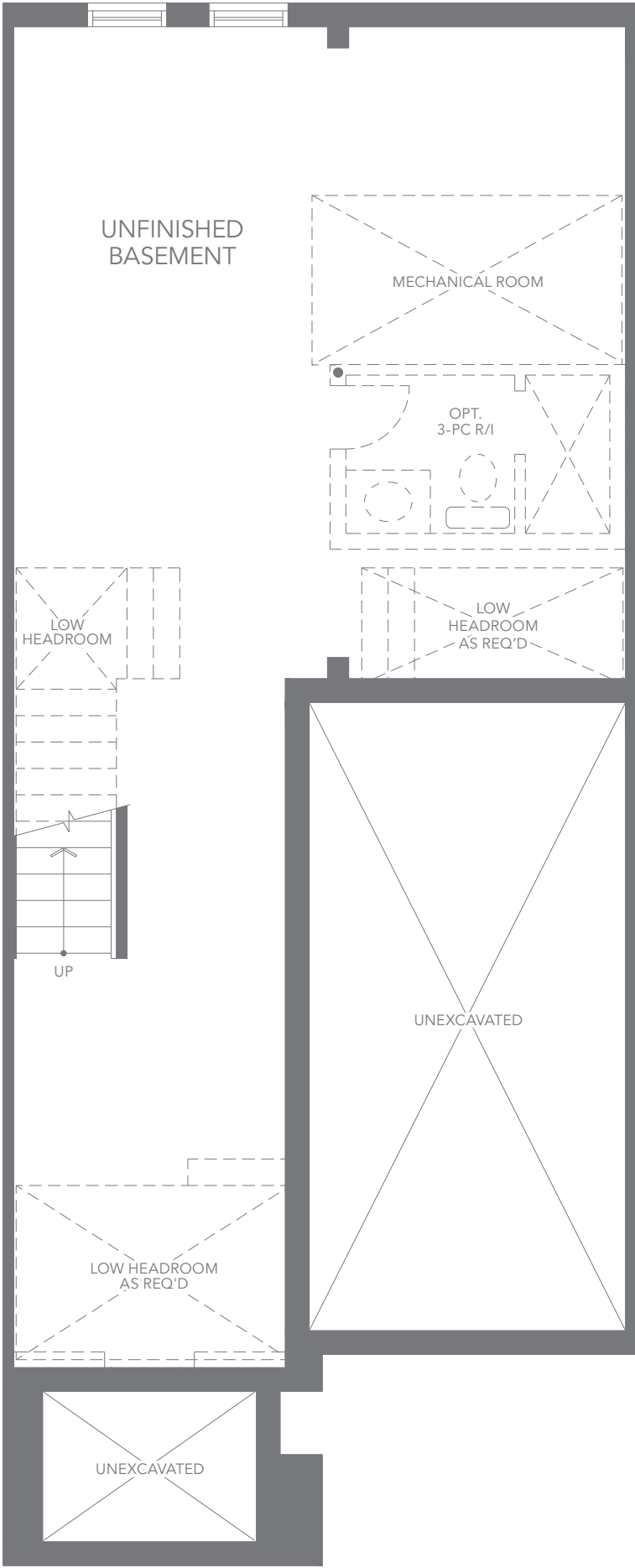
U2 ELEV. B1 BASEMENT FLOOR PLAN
