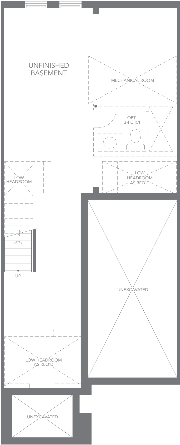
U2 ELEV. B2 BASEMENT FLOOR PLAN
