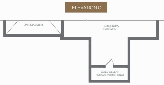
BASEMENT PLAN
