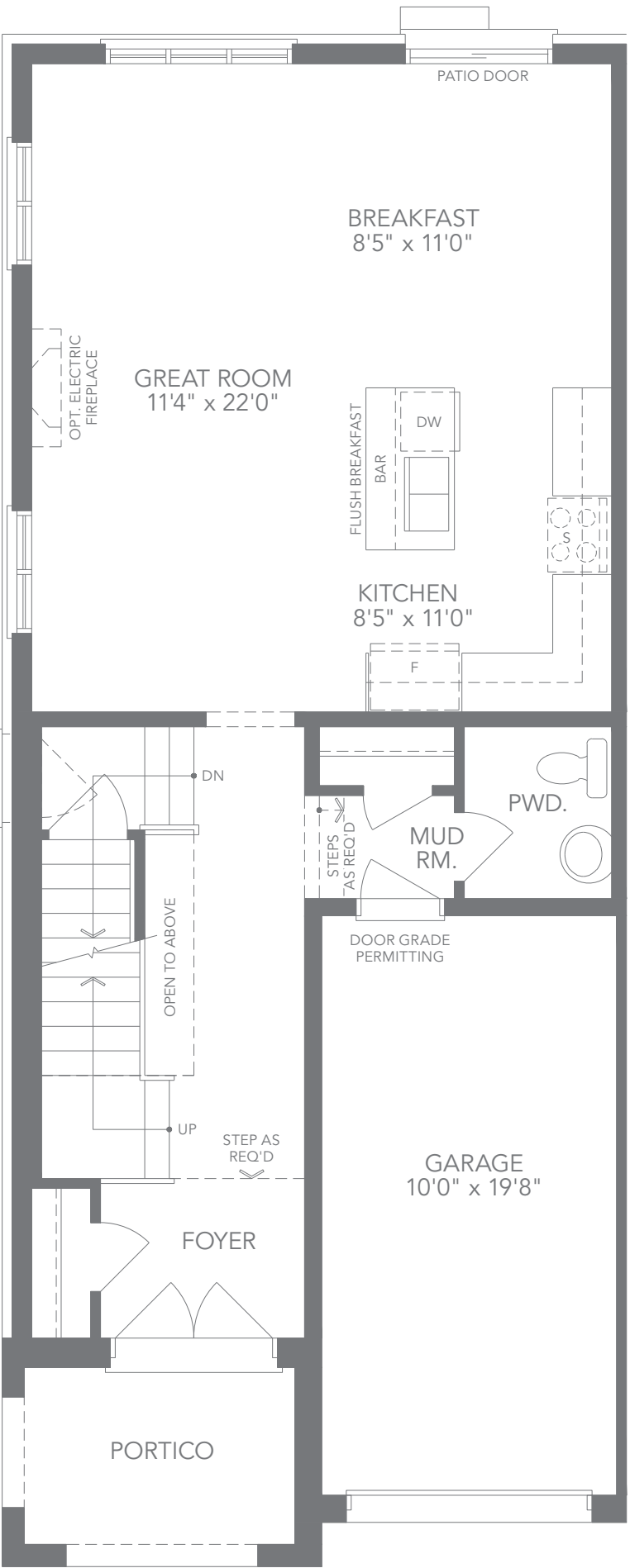
ELEV. B1 GROUND FLOOR PLAN
