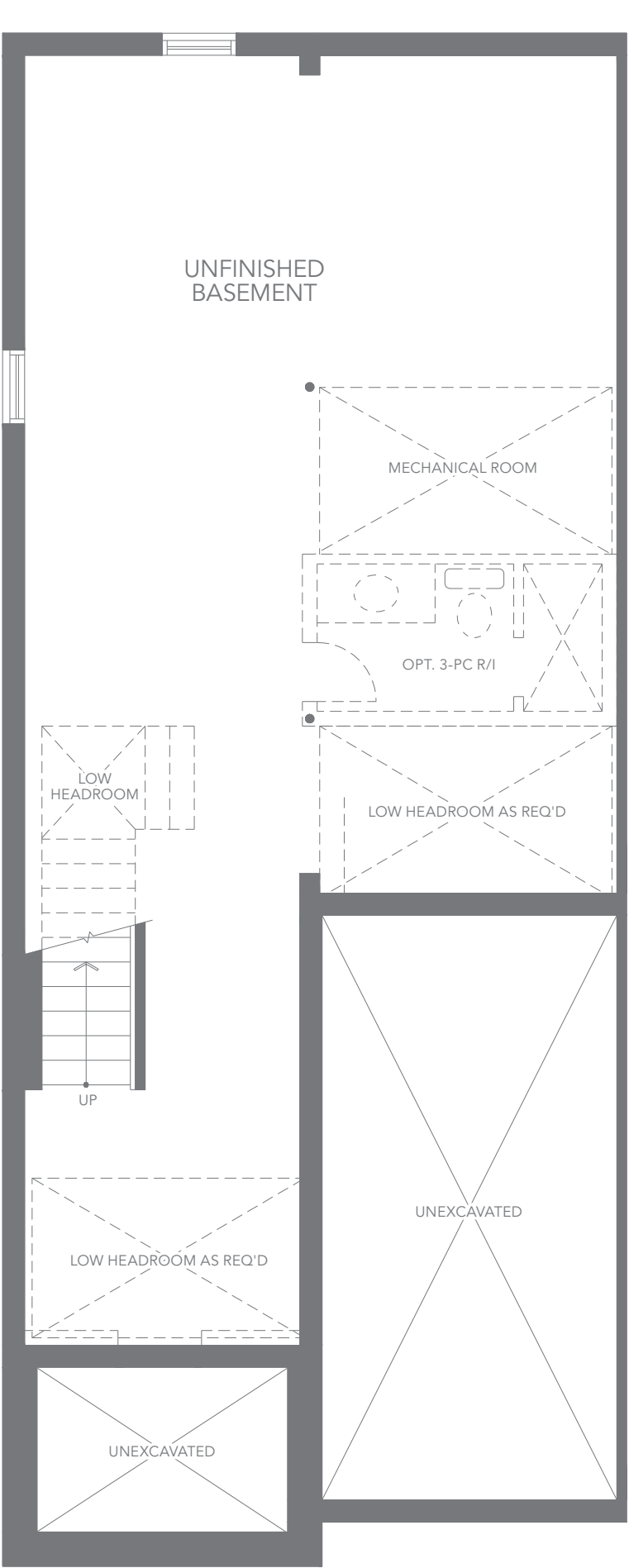
ELEV. A1 BASEMENT FLOOR PLAN
