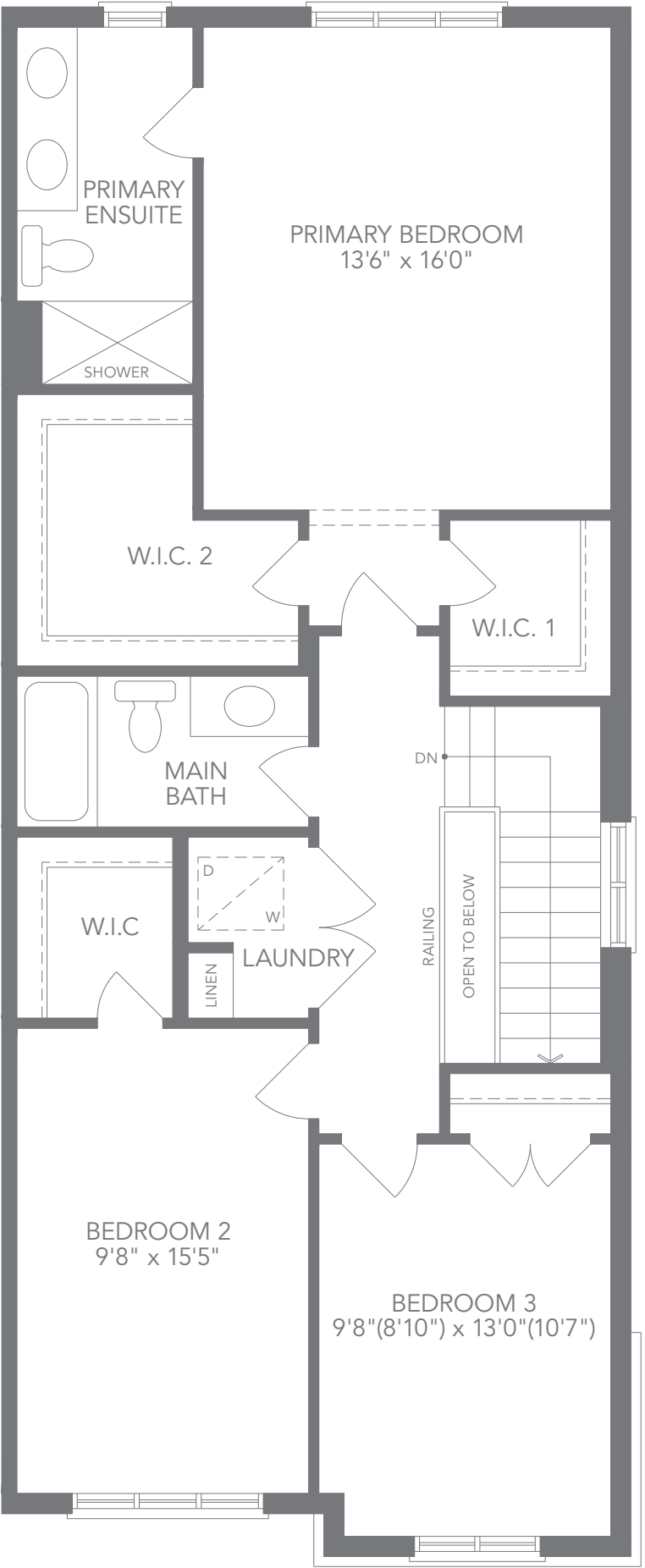
ELEV. B2 UPPER FLOOR PLAN
