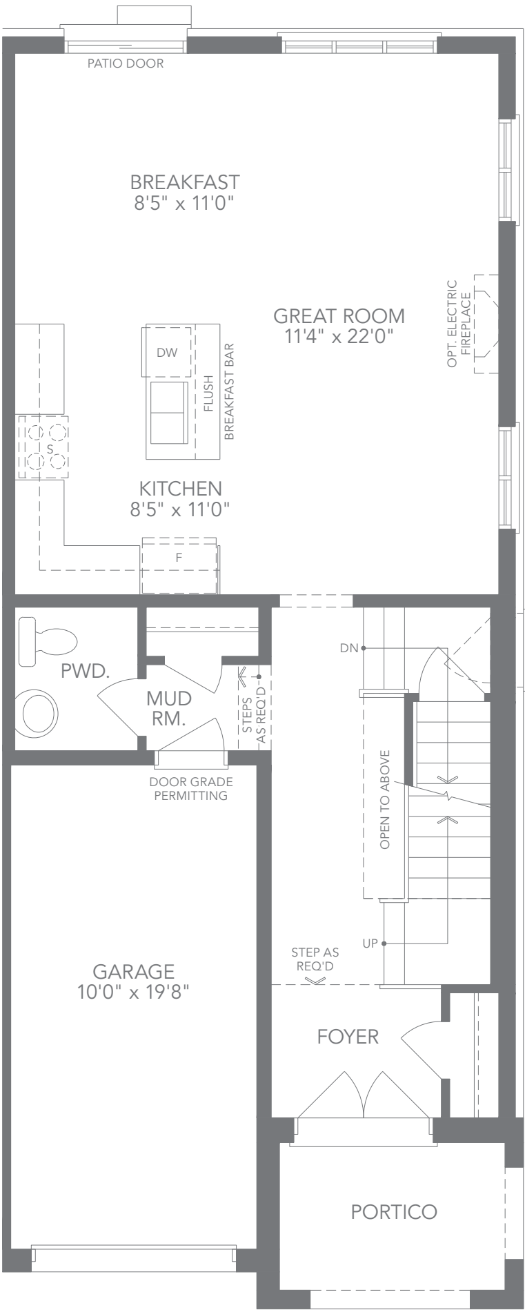
ELEV. B2 GROUND FLOOR PLAN
