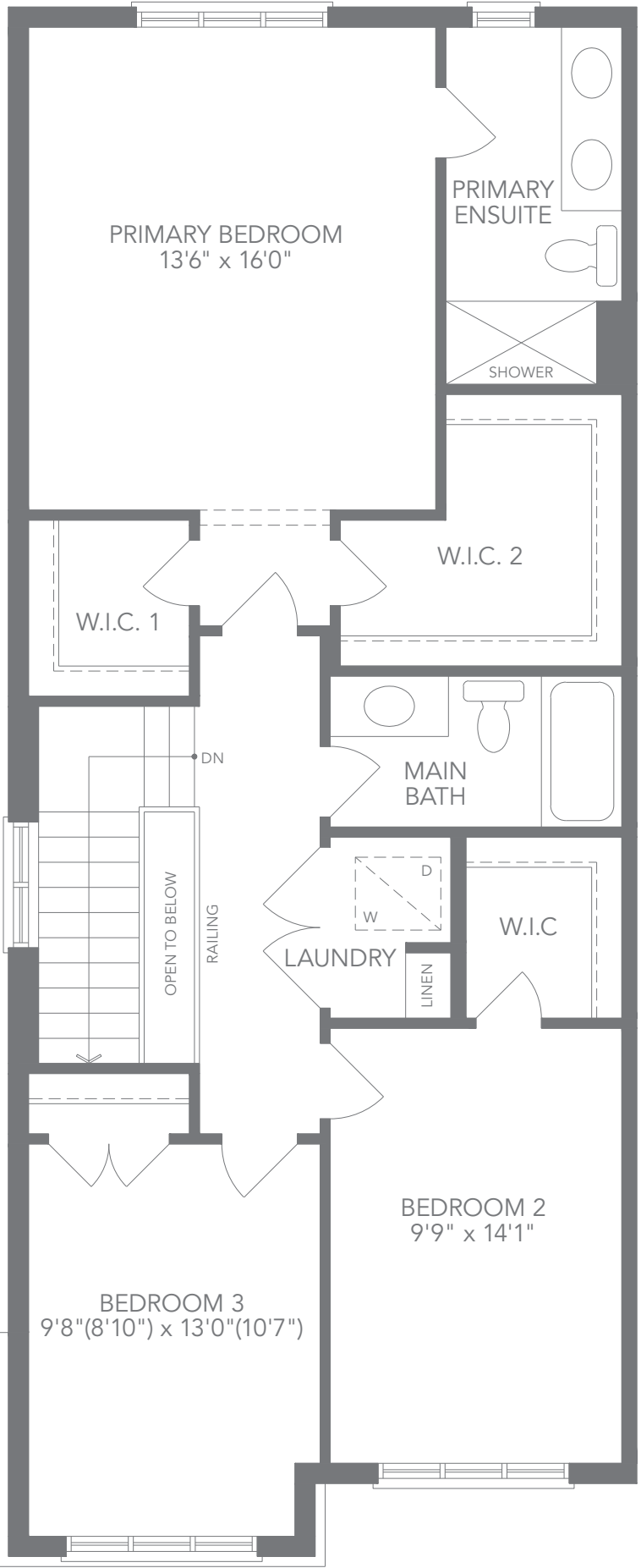
ELEV. B1 UPPER FLOOR PLAN
