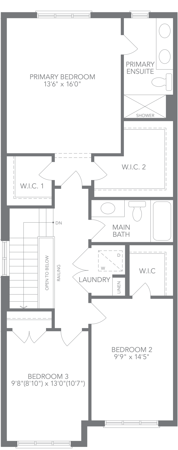
ELEV. A1 UPPER FLOOR PLAN
