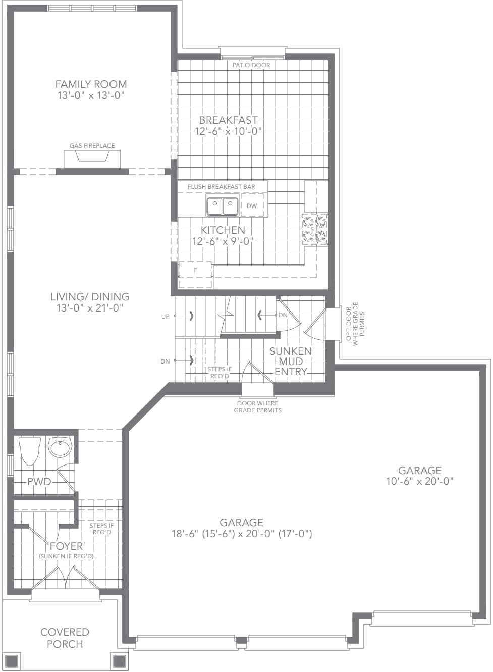
ELEV. A GROUND FLOOR PLAN
