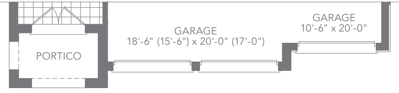
ELEV. C GROUND FLOOR PLAN
