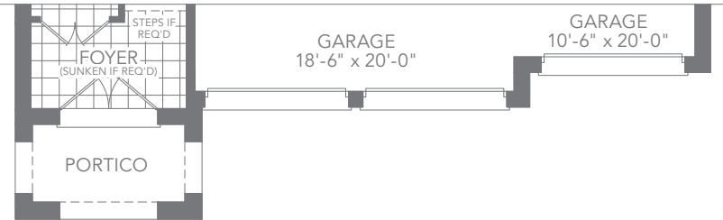
ELEV. B GROUND FLOOR PLAN
