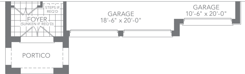
ELEV. C GROUND FLOOR PLAN
