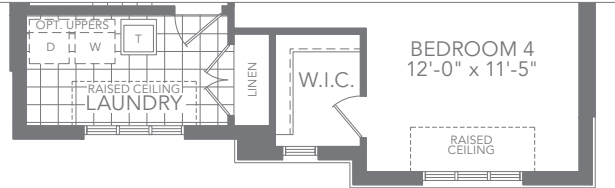
ELEV. C SECOND FLOOR PLAN
