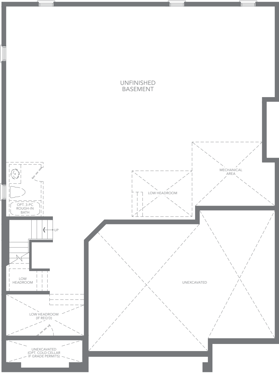
ELEV. A BASEMENT FLOOR PLAN
