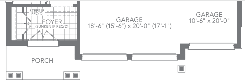
ELEV. C GROUND FLOOR PLAN
