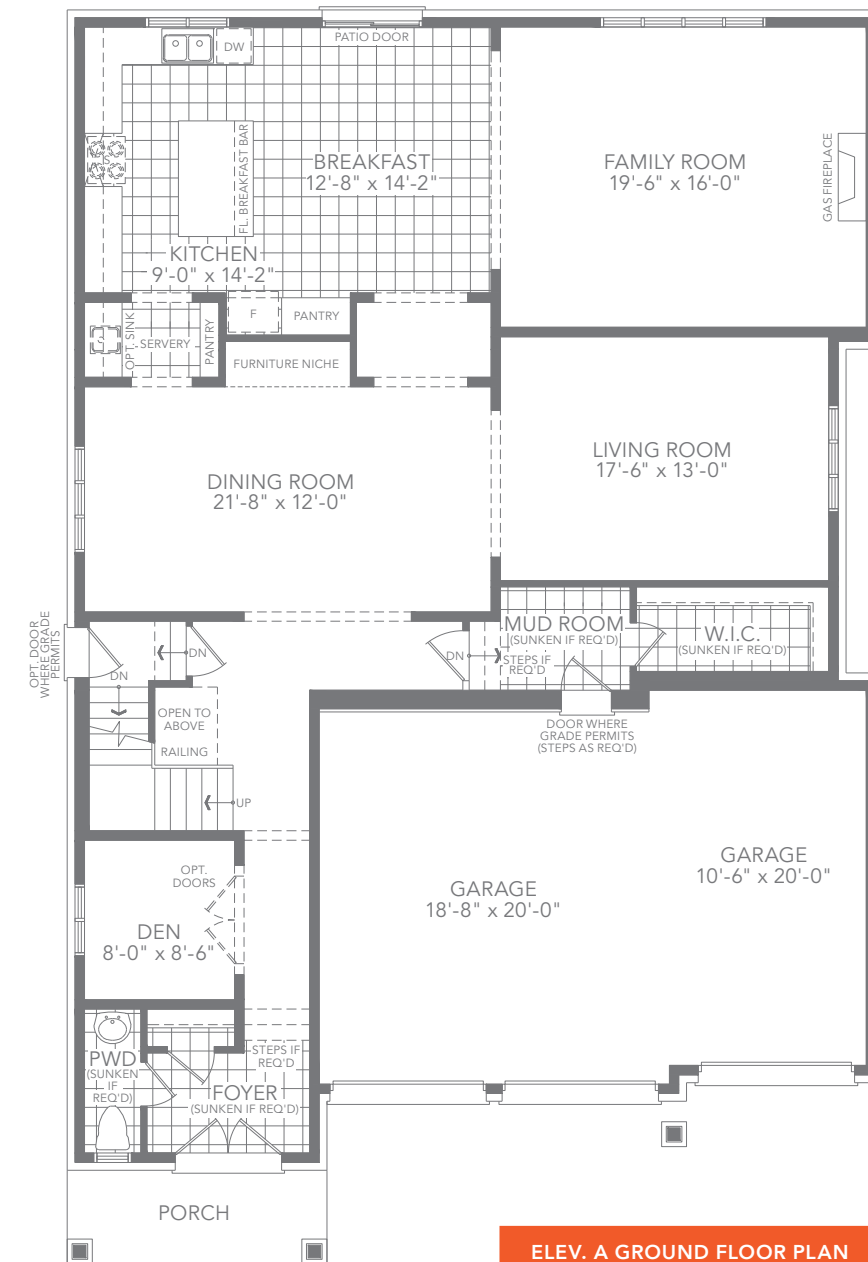
ELEV. A GROUND FLOOR PLAN
