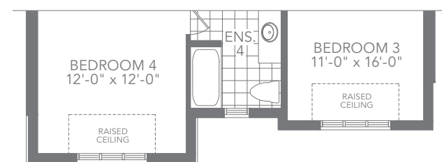
ELEV. C SECOND FLOOR PLAN
