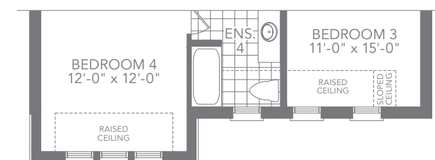
ELEV. B SECOND FLOOR PLAN
