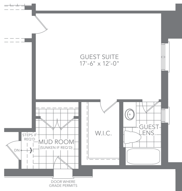
ELEV. B OPT. GROUND FLOOR PLAN
