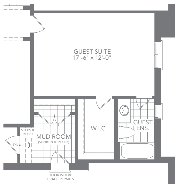
ELEV. C OPT. GROUND FLOOR PLAN
