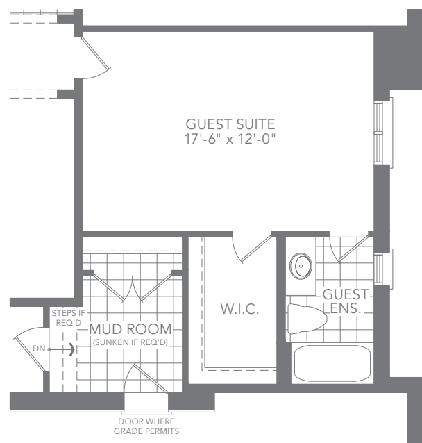
ELEV. D OPT. GROUND FLOOR PLAN
