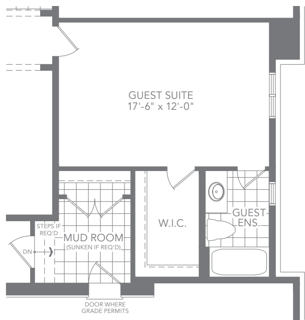
ELEV. A OPT. GROUND FLOOR PLAN
