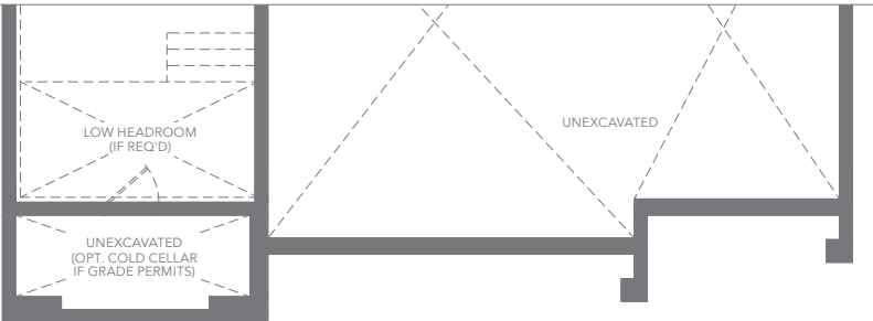
ELEV. C BASEMENT FLOOR PLAN
