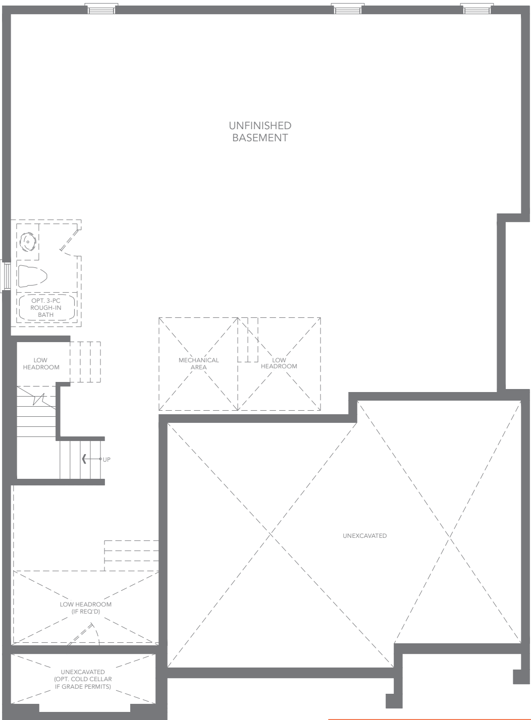
ELEV. A BASEMENT FLOOR PLAN
