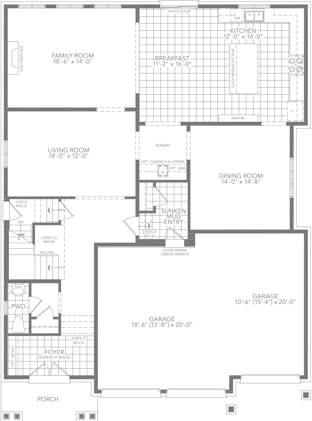
ELEV. A GROUND FLOOR PLAN
