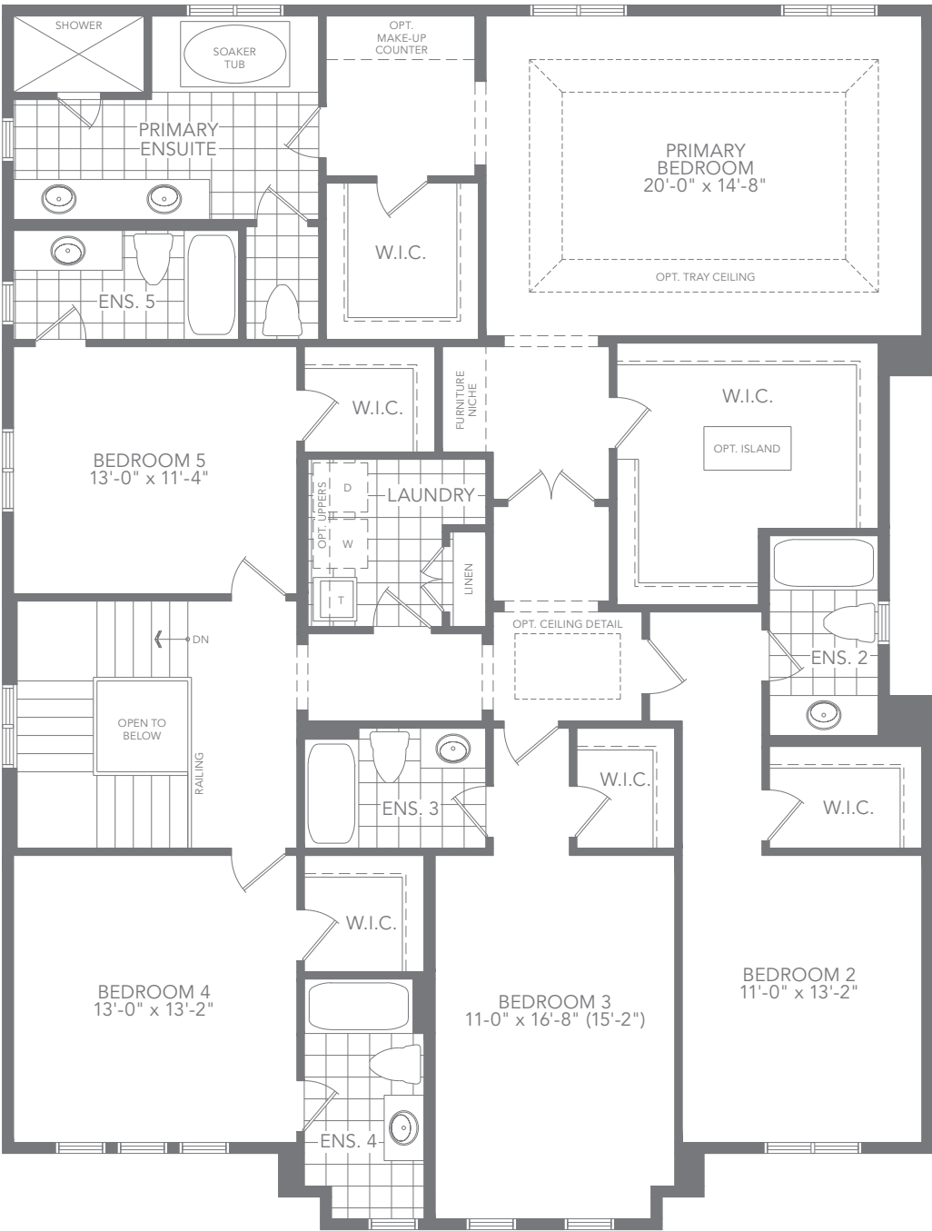
ELEV. A SECOND FLOOR PLAN
