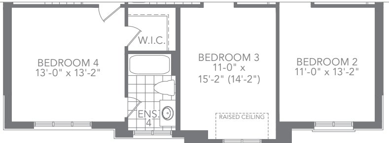
ELEV. B SECOND FLOOR PLAN
