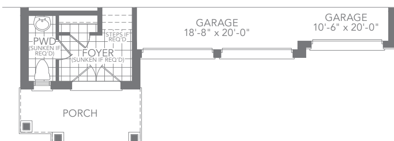
ELEV. D GROUND FLOOR PLAN
