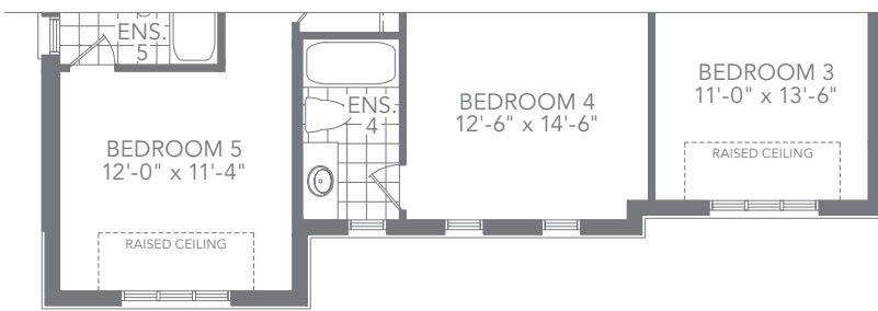
ELEV. C SECOND FLOOR PLAN
