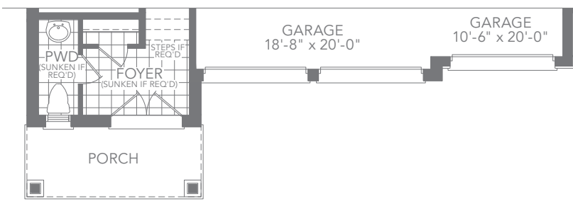
ELEV. C GROUND FLOOR PLAN
