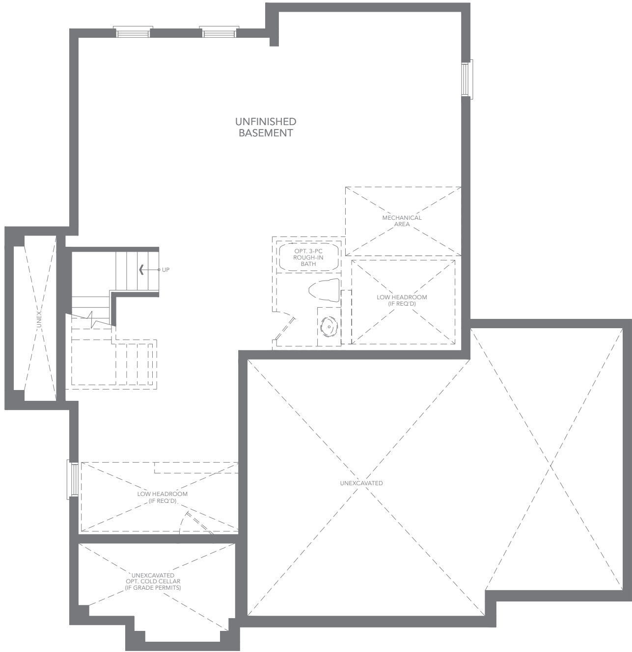
ELEV. B BASEMENT FLOOR PLAN
