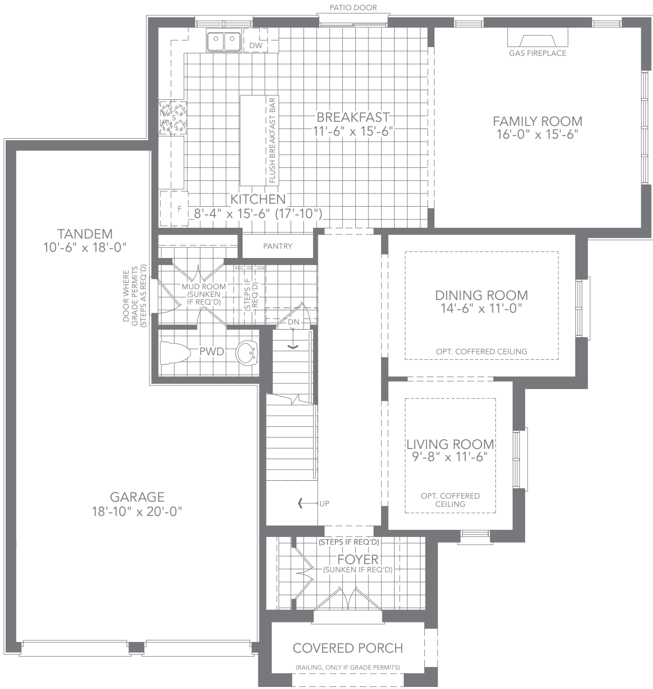
ELEV. C GROUND FLOOR PLAN
