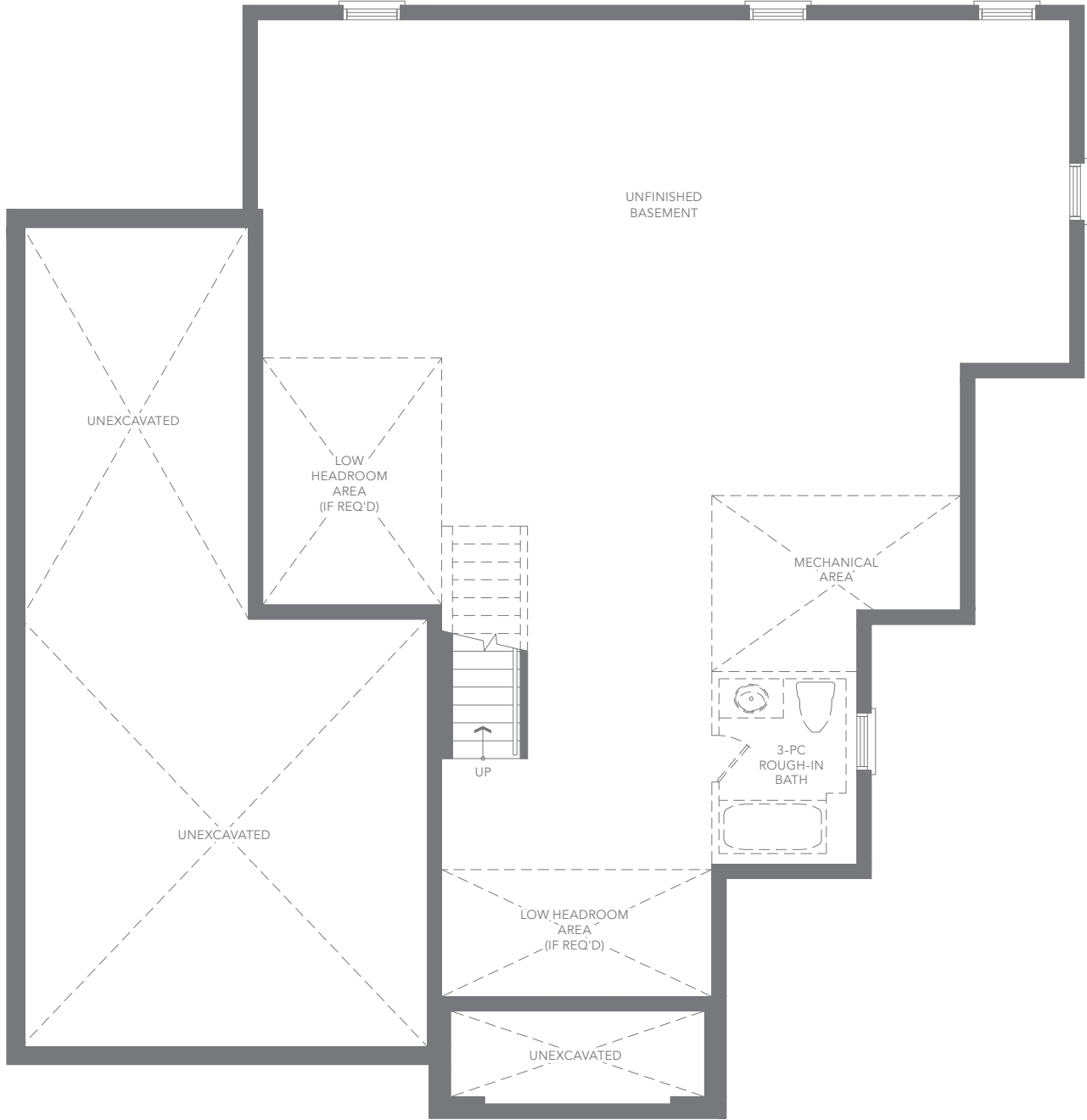
ELEV. C BASEMENT FLOOR PLAN
