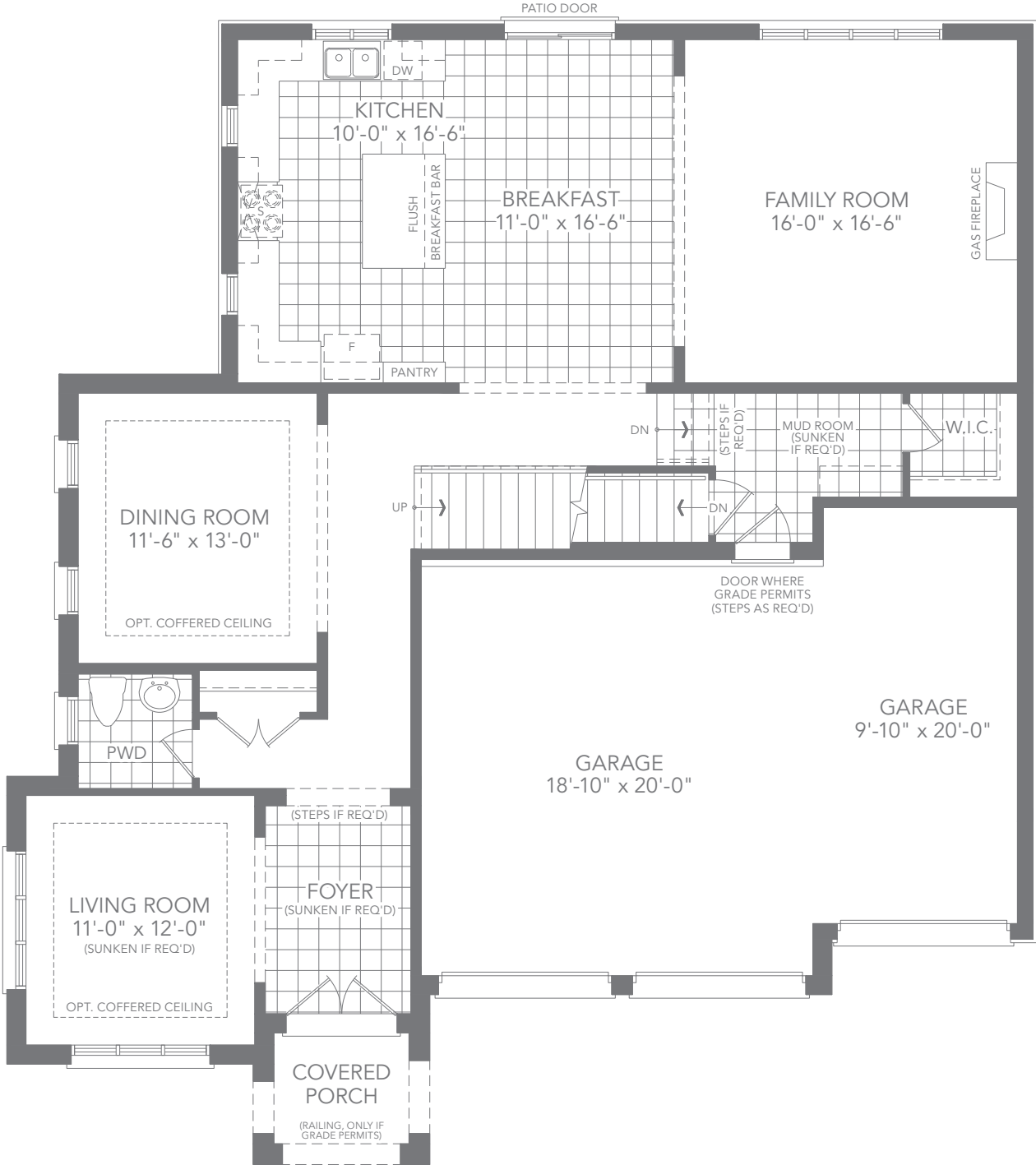
ELEV. C GROUND FLOOR PLAN
