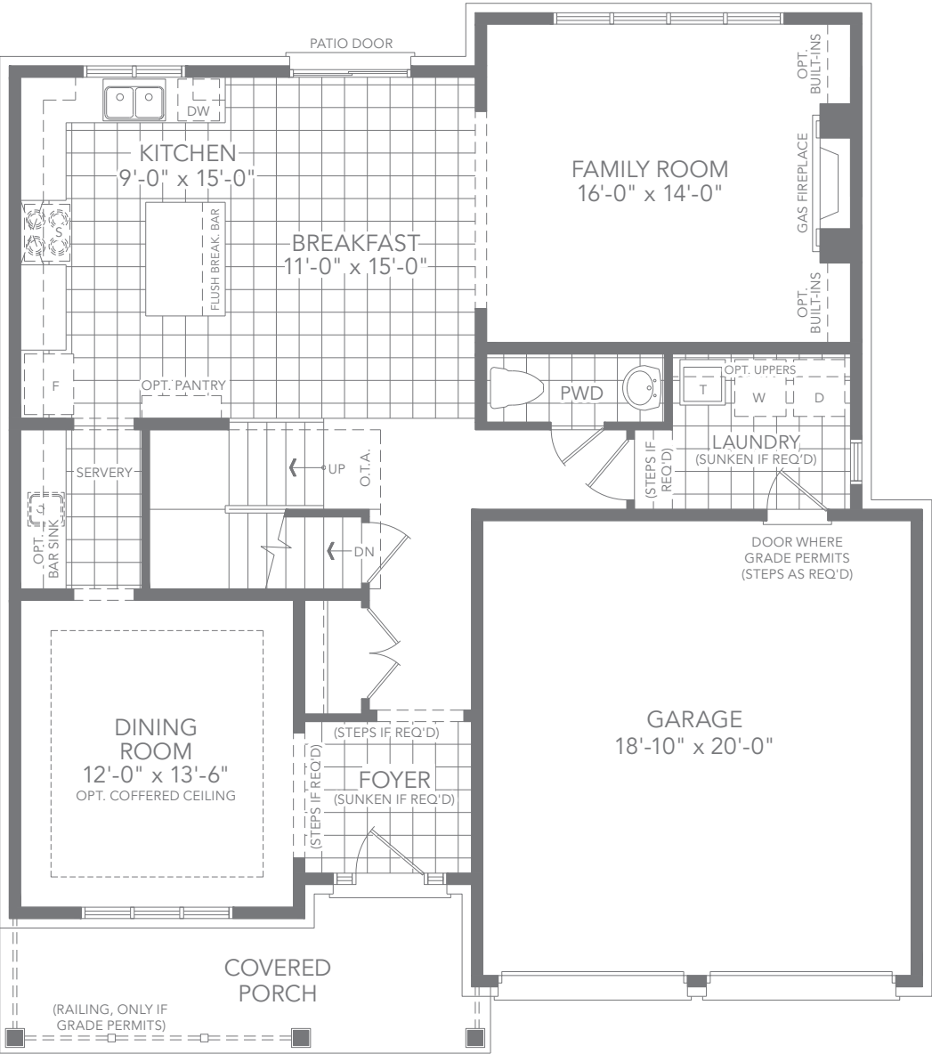
ELEV. A GROUND FLOOR PLAN
