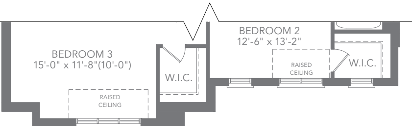
ELEV. C SECOND FLOOR PLAN
