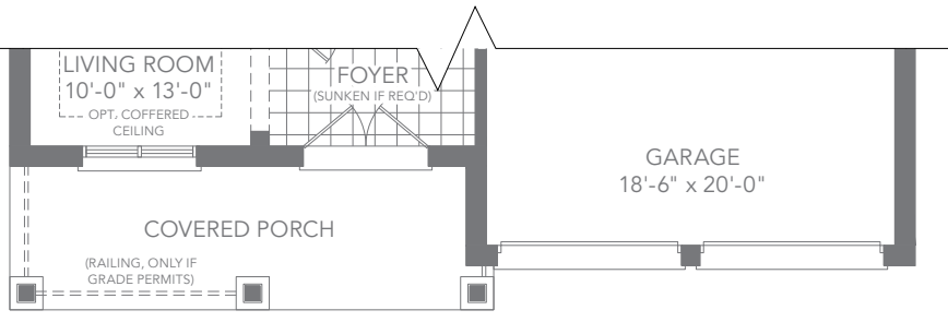
ELEV. C GROUND FLOOR PLAN
