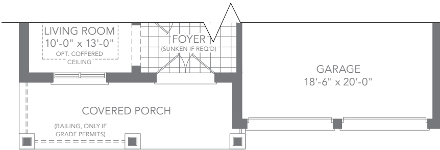
ELEV. B GROUND FLOOR PLAN
