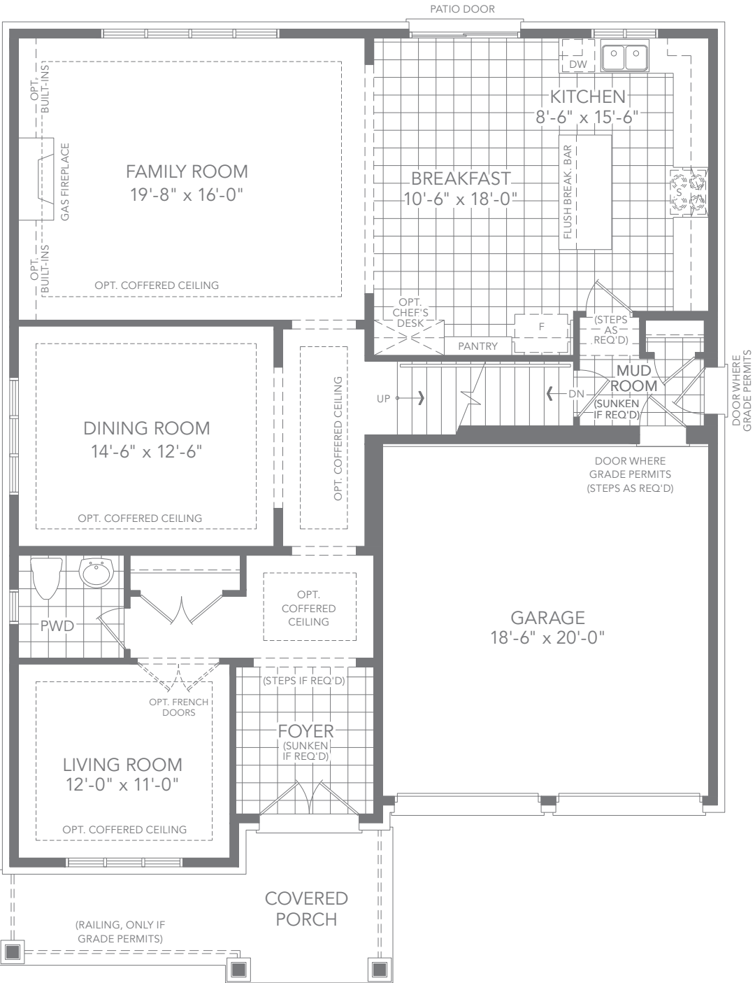
ELEV. A GROUND FLOOR PLAN
