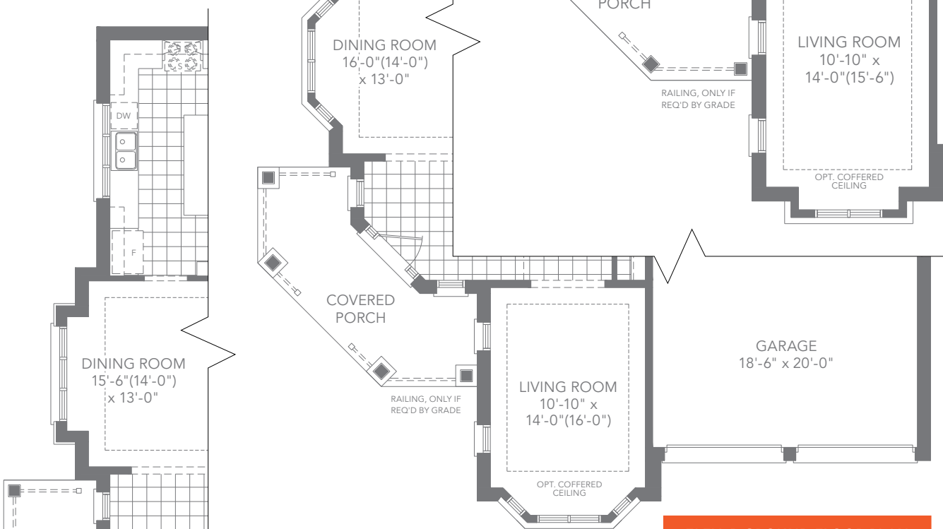
ELEV. B GROUND FLOOR PLAN
