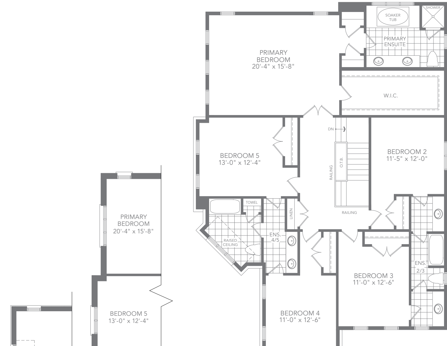
ELEV. A SECOND FLOOR PLAN
