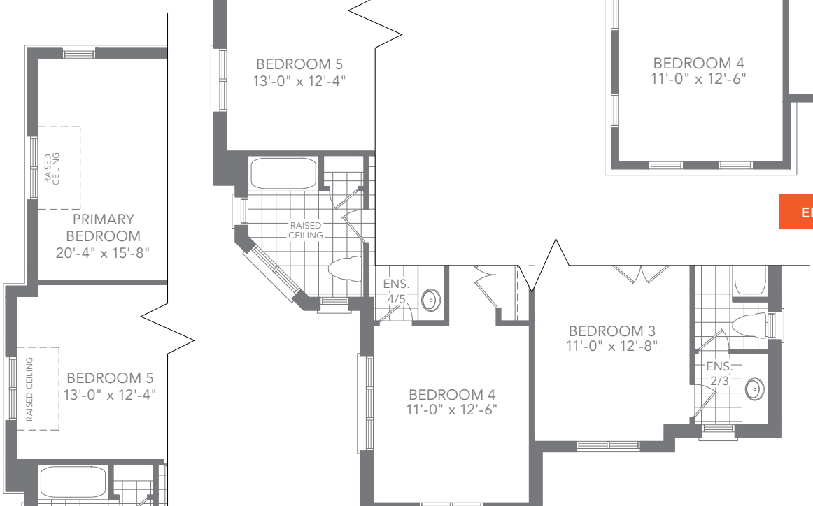
ELEV. B SECOND FLOOR PLAN
