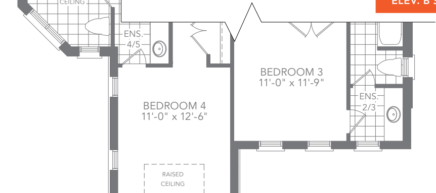
ELEV. C SECOND FLOOR PLAN
