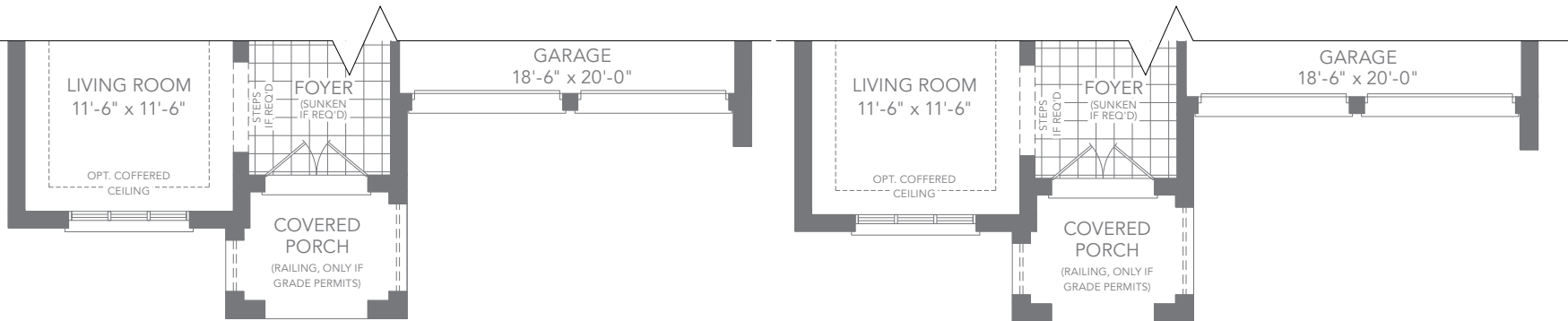
ELEV. B GROUND FLOOR PLAN
