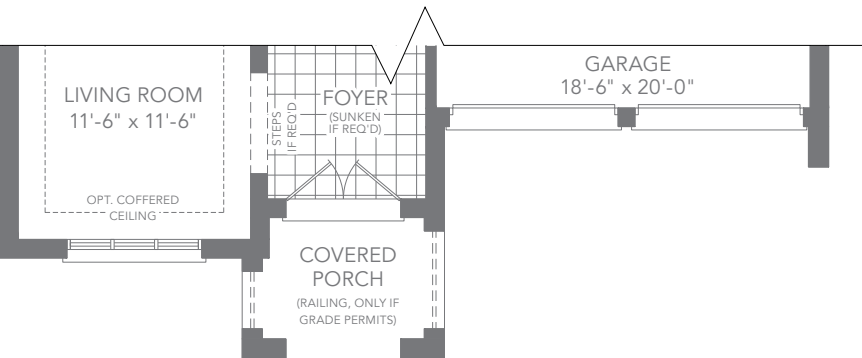
ELEV. C GROUND FLOOR PLAN
