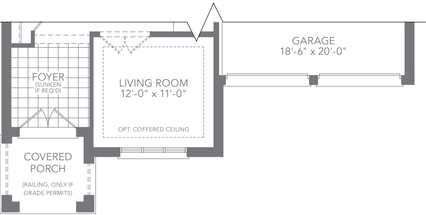
ELEV. C GROUND FLOOR PLAN
