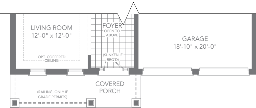
ELEV. B GROUND FLOOR PLAN
