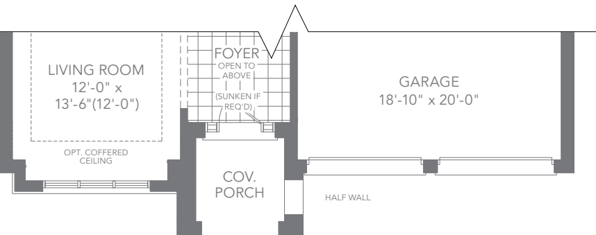
ELEV. C GROUND FLOOR PLAN
