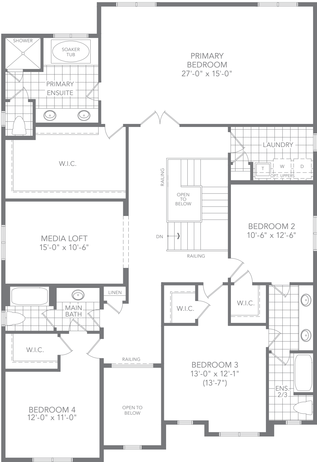
ELEV. A SECOND FLOOR PLAN
