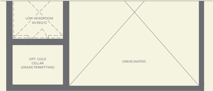
BASEMENT PLAN
