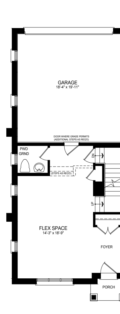
Ground Floor Elev. A
