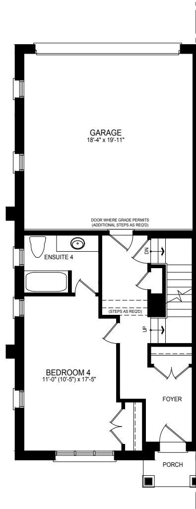
Opt. Ground Floor Elev. A
