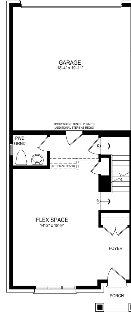
Modified Ground Floor Elev. A
