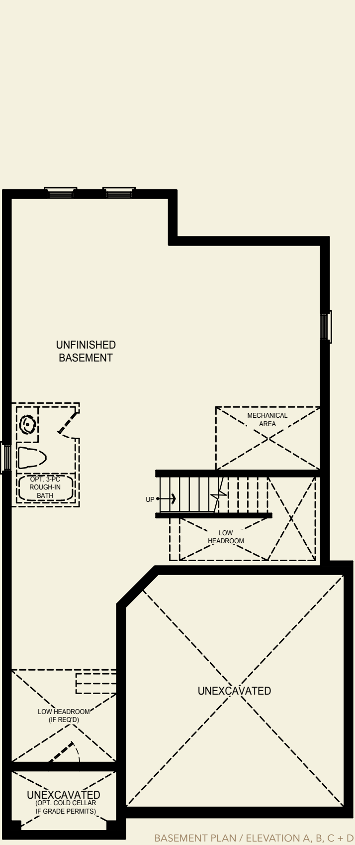
BASEMENT PLAN / ELEVATION A, B, C + D
