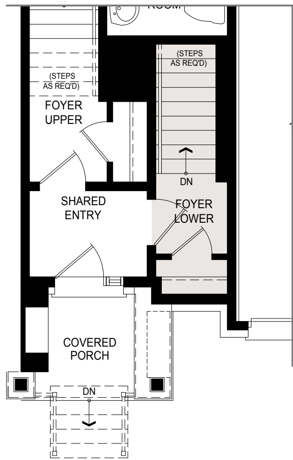
MAIN LEVEL SHARED ENTRY
