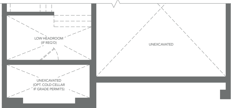
ELEVATION C
