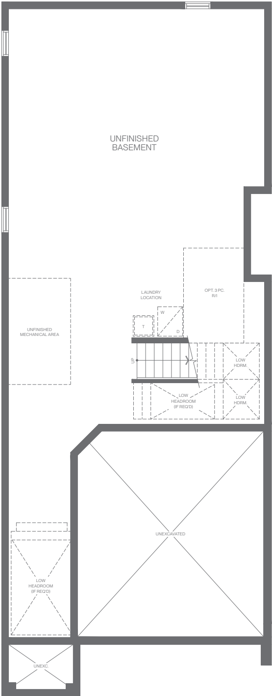
BASEMENT PLAN / ELEVATION B
