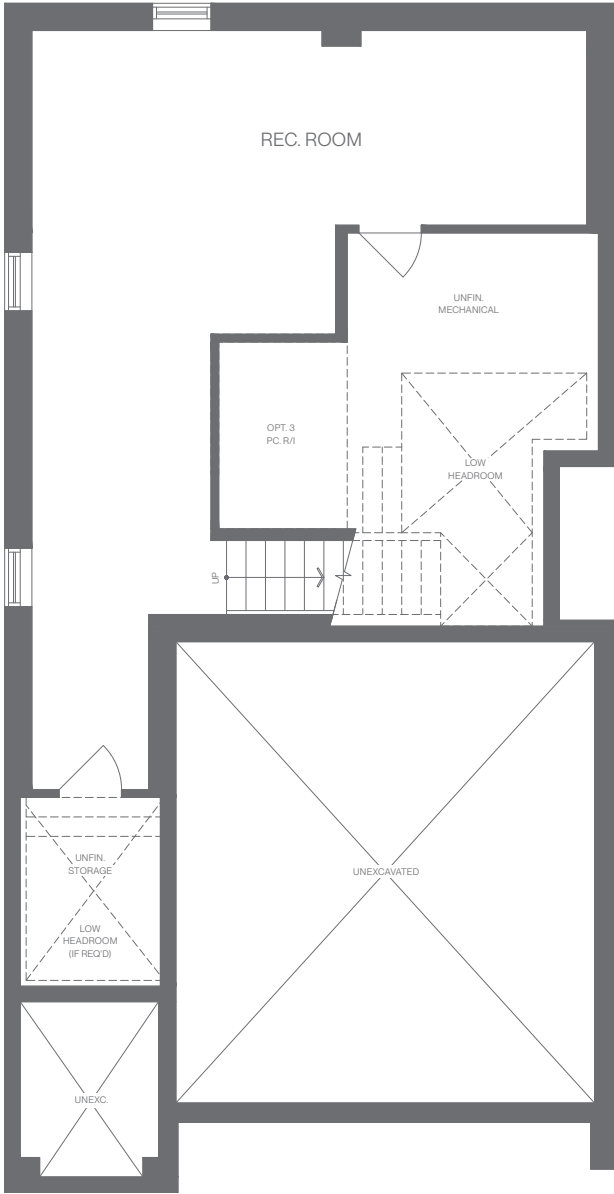
FINISHED BASEMENT PLAN / ELEVATION A
