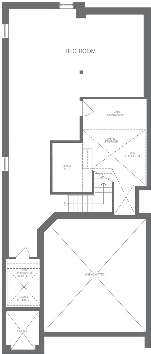
FINISHED BASEMENT PLAN / ELEVATION A
