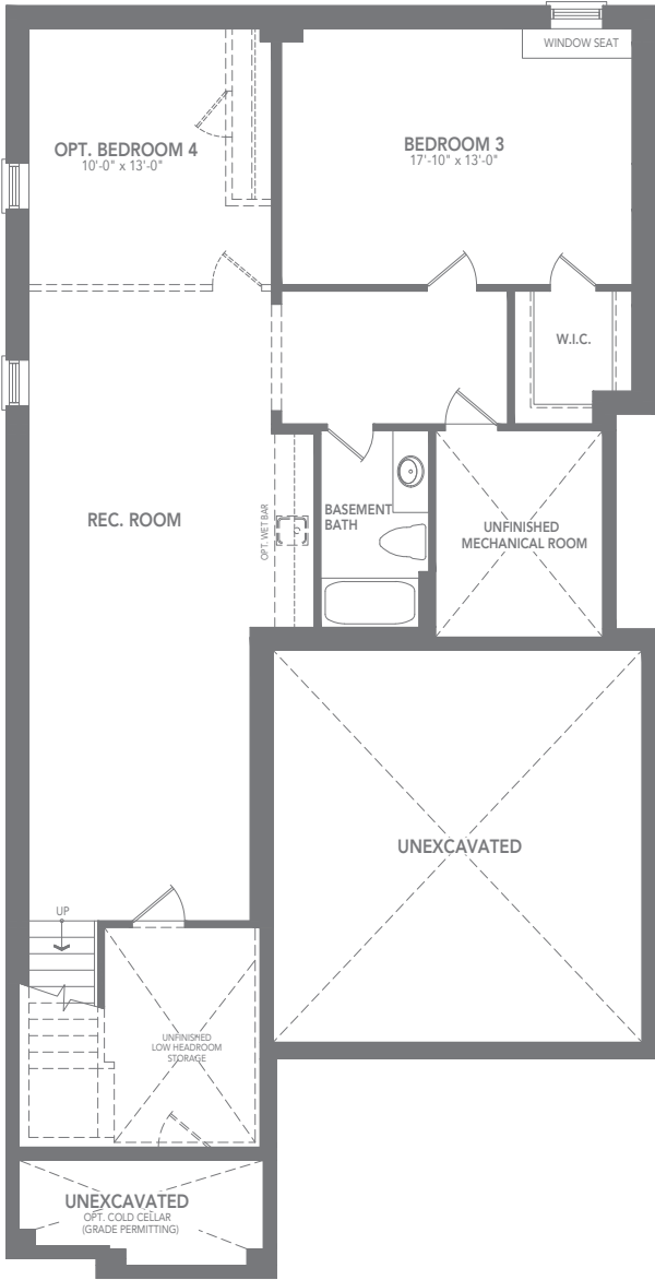
FINISHED BASEMENT PLAN / ELEVATION B
