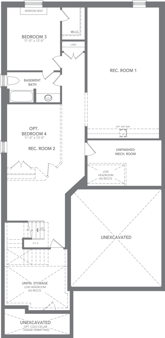
FINISHED BASEMENT PLAN / ELEVATION B
