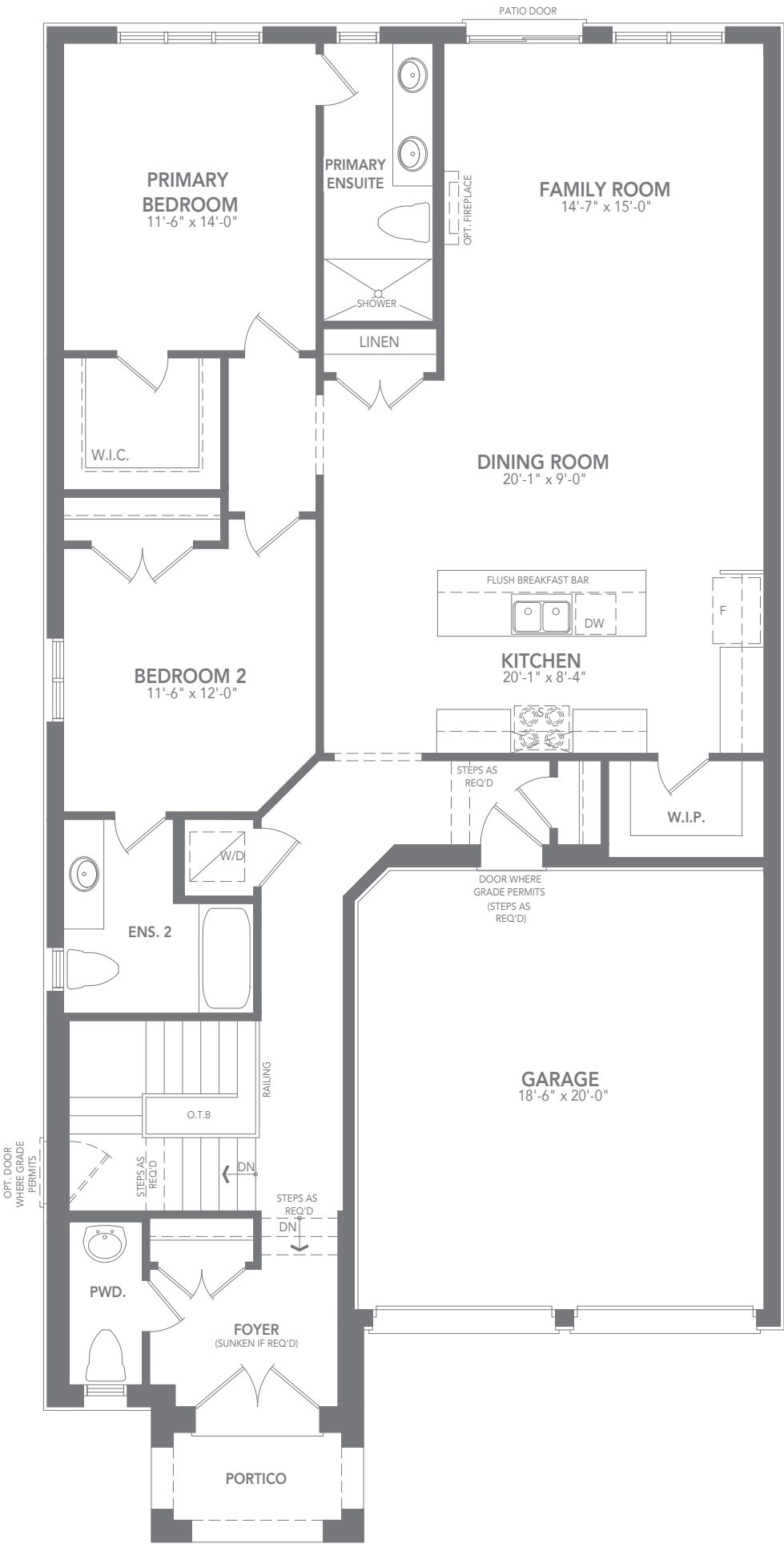
GROUND FLOOR PLAN ELEVATION B
